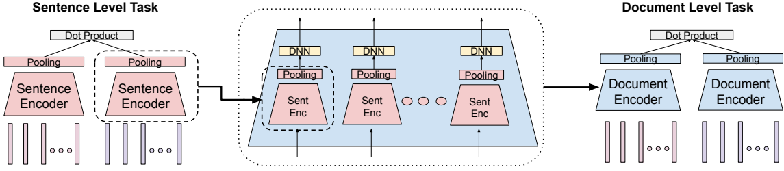
Figure 2: Illustration of the DNN \rightarrow pooling version of the Hierarchical Document Encoder (HiDE). Each sentence is processed by our Transformer based encoding model with the final sentence-level embedding being produced by pooling across the last layer’s positional heads. Document-level embeddings are composed by pooling across the sentence-level embeddings after each sentence embedding has been adapted by additional feed-forward layers.
