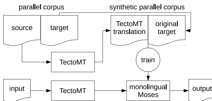
Figure 3: PhraseFix
