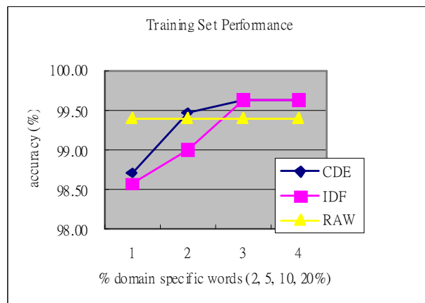
Figure 1. Training Set Performance
