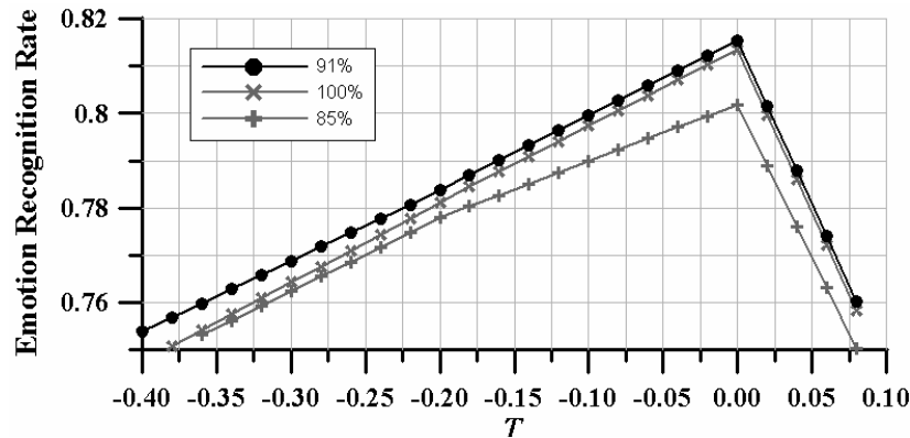
Figure 4. Emotion recognition rates for acoustic features under different PCA thresholds. The black line indicates the results obtained when R^2 = 91\% , and the two gray lines indicate the results obtained when R^2 = 85\% and 100\% .
