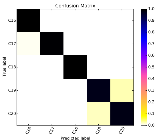
Figure 1: Confusion Matrix: Century Classification
