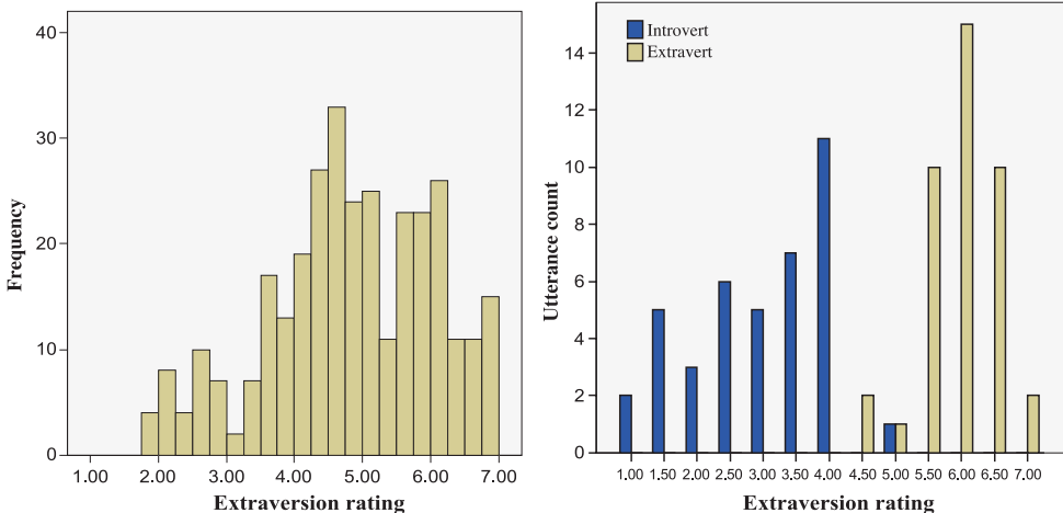
(a) Distribution of extraversion scores on the random sample.
