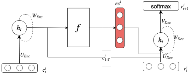
Figure 1: Architecture Diagram of Extended Encoder Decoder Model.
