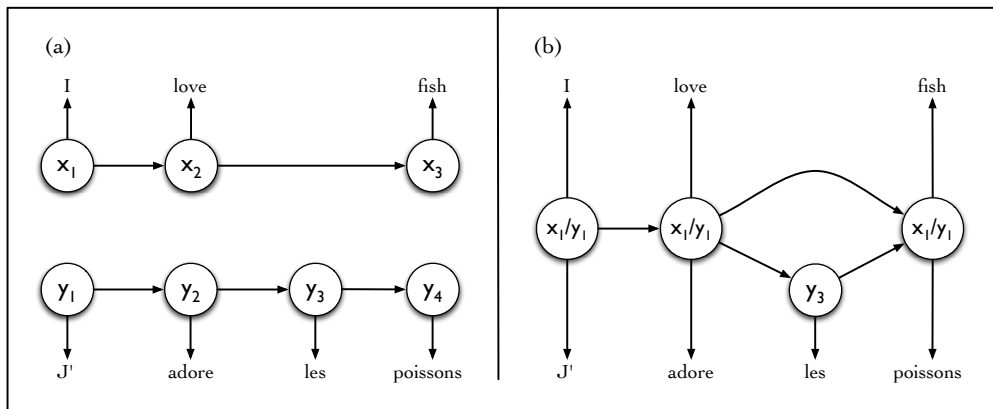
Figure 1: (a) Graphical structure of two standard monolingual HMM's. (b) Graphical structure of our bilingual model based on word alignments.
