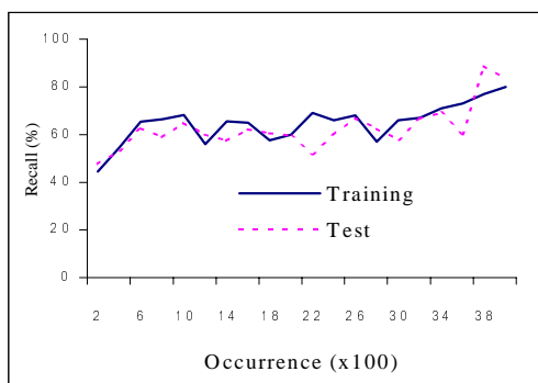
Figure 4: Recall-Occurrence Relationship
