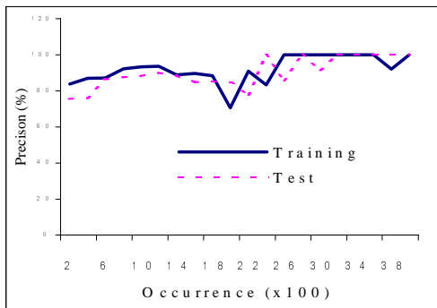
Figure 3: Precision-Occurrence Relationship
