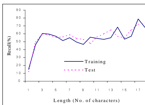
Figure 6: Precision-Length Relationship
