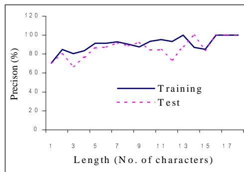
Figure 5: Precision-Length Relationship
