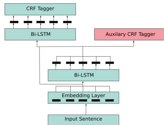
Figure 1: The overall architecture where the STL model contains all of the green layers and the MTL uses the additional pink auxiliary CRF tagger. The second Bi-LSTM has a skip connection from the embedding layer which concatenates the word embeddings with the output from the first Bi-LSTM.
