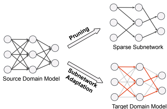
Figure 1: Domain adaptation with subnetworks of the source domain model. Various pruning methods can be used to find sparse subnetworks. Only the parameters (red arrow \rightarrow ) of the subnetworks are updated. The rest (grey arrow \rightarrow ) are frozen but used in inference.
