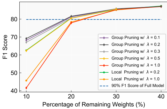
Figure 4: Pruning with and without self-attention head importance. Horizontal line indicates 90% F1 score of the full model. Sparsity percentage are relative to BERT-base with 84M parameters. \lambda is importance factor. For both local pruning and group pruning, attention head importance scores help identify better lottery networks at high sparsity levels.
