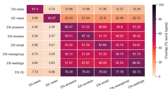
Figure 1: Domain overlap between target (x-axis) and source training (y-axis) domains (DE: German, DA: Danish, EN: proposed dataset EWT-NNER).
