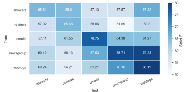
Figure 2: In-language cross-domain evaluation.
