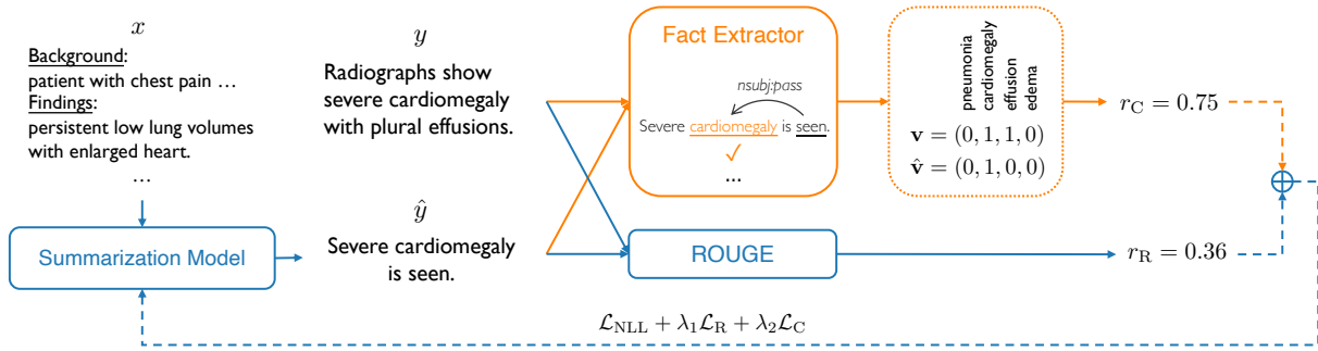
Figure 2: Our proposed training strategy. Compared to existing work which relies only on a ROUGE reward r_R , we add a factual correctness reward r_C which is enabled by a fact extractor. The summarization model is updated via RL, using a combination of the NLL loss, a ROUGE-based loss and a factual correctness-based loss. For simplicity we only show a subset of the clinical variables in the fact vectors \mathbf{v} and \hat{\mathbf{v}} .
