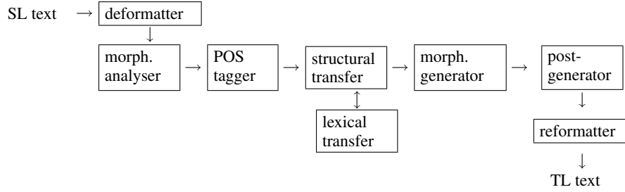
Figure 1: The eight modules of the shallow-transfer machine translation system
