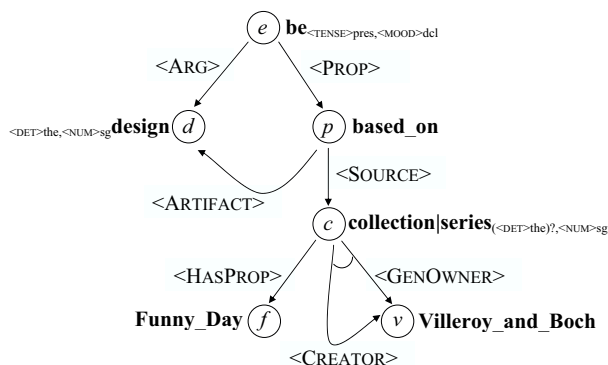
Figure 1: Simplified disjunctive semantic dependency graph from the COMIC dialogue system, for the eight paraphrases The design (is|’s) based on (the Funny Day (collection|series) by Villeroy and Boch | Villeroy and Boch’s Funny Day (collection|series)) .
