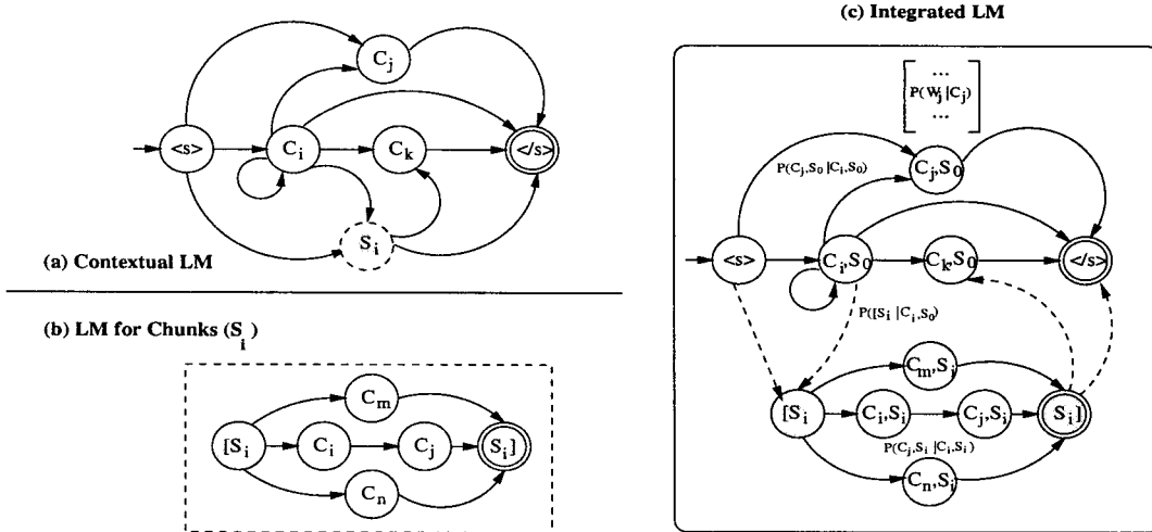
Figure 1: Integrated Language Model for Tagging and Chunking.
