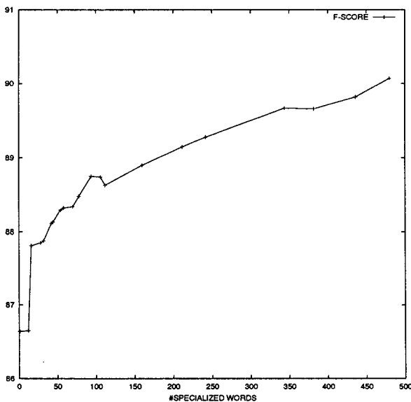
Figure 2: F-score as a function of the number of specialized words in the ILM
