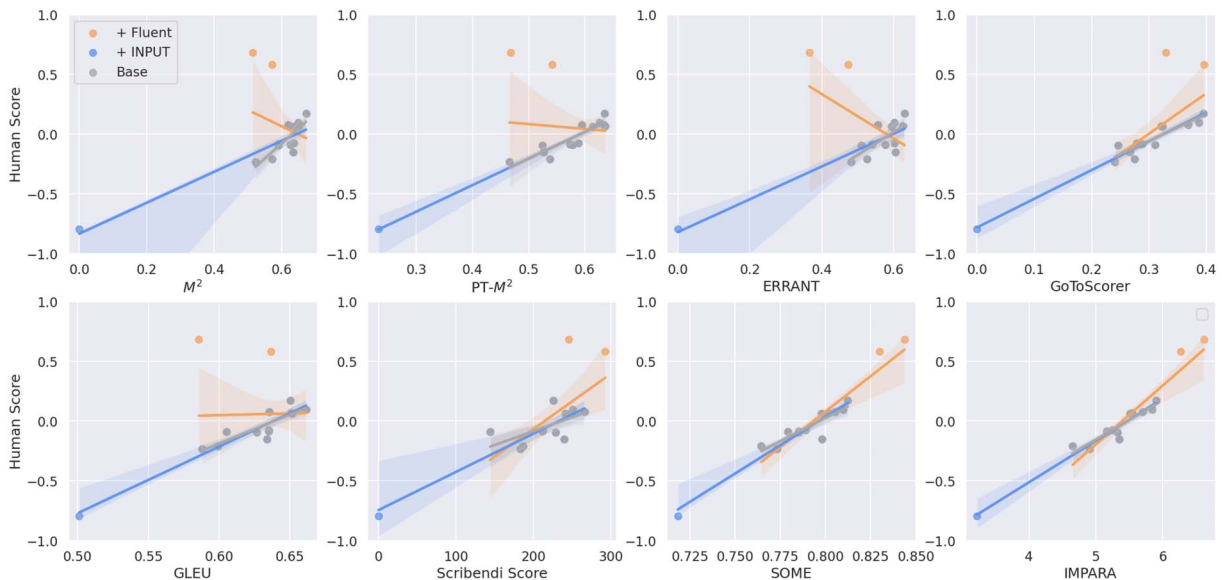
Figure 3: Scatter plots of the human score and the metric score. ‘‘Base’’ indicates the 12 systems excluding uncorrected sentences (INPUT) and fluent sentences (REF-F, GPT-3.5). Each line represents a regression line, and the shaded area indicates the size of the confidence interval for the estimated regression, obtained using bootstrap. Comparing the orange and blue regression lines to the gray regression line allows us to observe the degree of influence of each outlier on the distribution trend. For example, the leftward tilt of the orange regression lines for M^2 , PT-M^2 , ERRANT, and GLEU indicates a negative impact from fluent sentences as outliers.
