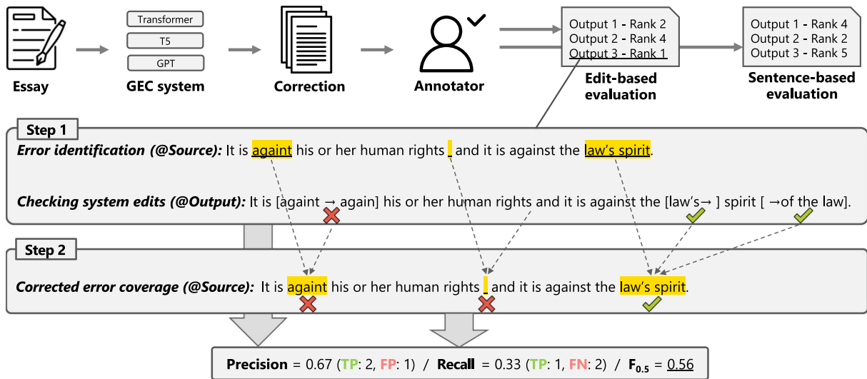
Figure 2: An overview of the annotation flow and an example of edit-based human evaluation. In Step 1, the annotator identifies errors in the source. Then, they categorize each edit in the output as either valid or not. In Step 2, the annotator determines whether each edit in the output effectively corrects the errors found in Step 1. TP, FP, and FN represent True Positive, False Positive, and False Negative, respectively.
