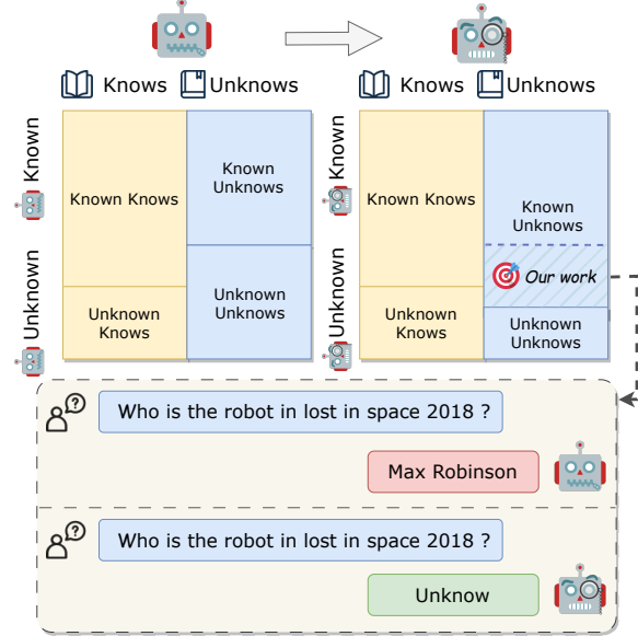
Figure 1: The evolution of the Known-Unknown Quadrant. The yellow portion represents the model’s parametric knowledge. Our method increases the “Known Unknowns”, helping the model recognize and articulate its knowledge limitations.
