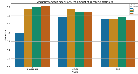
Figure 4: Accuracy of each model with a varying number of in-context examples given before generation.
