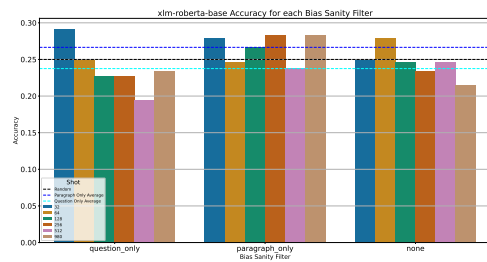
Figure 5: The results of fine-tuning XLM-Roberta on the Armenian QA dataset with a varying number of training samples while using only paragraphs, questions or random data.
