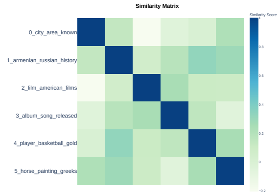
Figure 2: BERTopic embeddings similarity heatmap for the top 6 frequent topics in the mined English paragraphs.
