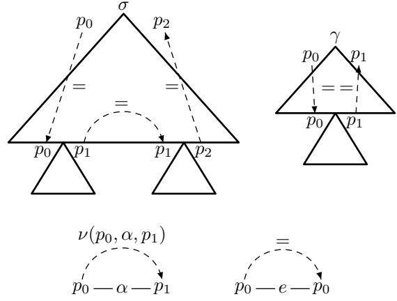
Figure 2: Information transport in the first and third components of the states in our Bar-Hillel construction.
