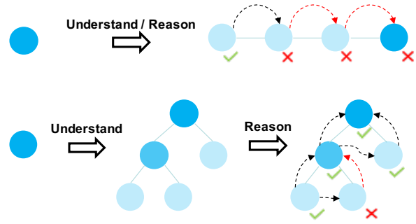
Figure 1: In chain-of-thought reasoning, the error in one step propagates to the final answer due to limited sight. Tree-of-thought reasoning can eliminate this problem by reconsidering the answer on the non-leaf nodes. The red edge means error propagation.
