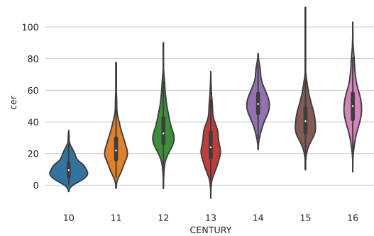
Figure 3: Violinplot of CER per century
