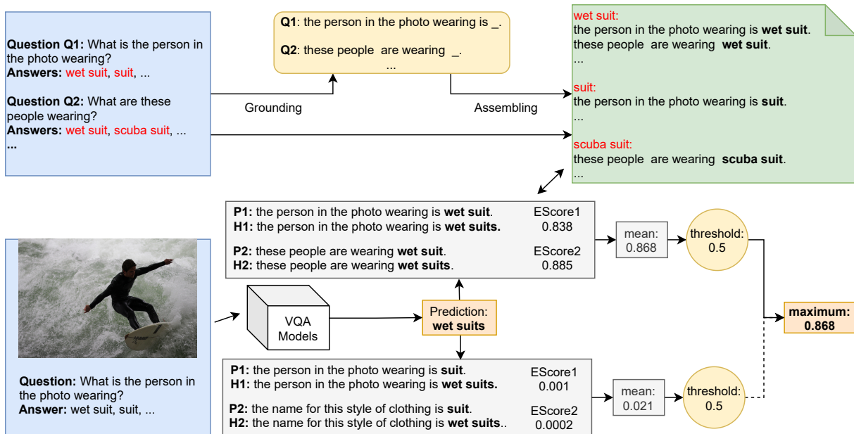
Figure 7: This example calculates the entailment score of provided answer “wet suit” and our prediction “wet suits”. We first ground all questions into statements with a reserved position “_”. Then, we congregate all the grounded statements by the provided answer. We replace the “_” with the provided and predicted answer separately as the premise and hypothesis to get the entailment score. The entailment score of a provided answer and a prediction is calculated as the mean of all the entailment scores under that answer in the assembling list. We take 0.5 as the threshold, and use the maximum as the final entailment score.
