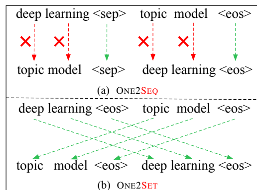
Figure 1: An example of ground-truth keyphrases (upper) and predictions (lower) under ONE2SEQ and ONE2SET training paradigm. For the ONE2SEQ training paradigm, although the predictions are correct in each keyphrase, they will still be considered wrong due to the shift in keyphrase order, and the model will receive a large penalty.
