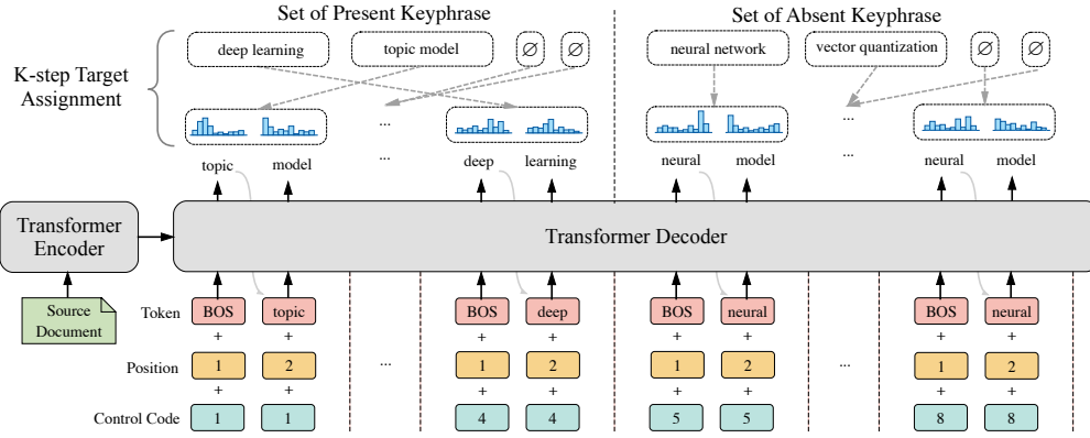
Figure 2: Architecture of SETTRANS model with N learned control codes as input conditions. A K -step target assignment mechanism is used during training, where we first predict K words for each code, and then find an optimal allocation among the predictions and targets. In the figure, N = 8 and K = 2 are used.
