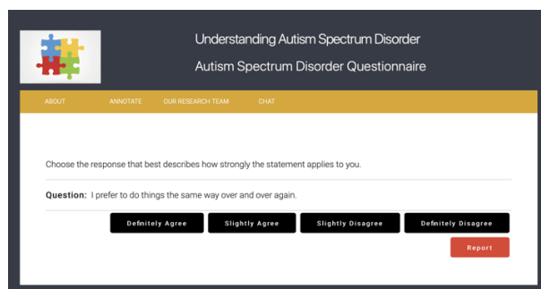
Figure 11: Questionnaire task
