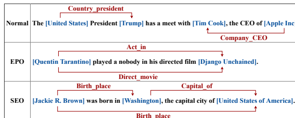
Figure 1: Examples of Normal , EntityPairOverlap (EPO) and SingleEntityOverlap (SEO) overlapping patterns.
