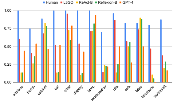
Figure 8: Human evaluation of L3GO, ReAct-B, Reflexion-B, and GPT-4 on ShapeNet-13. ‘Human’ refers to the original human-designed ShapeNet meshes. We observed a pattern similar to that in GPT-4V’s evaluation.
