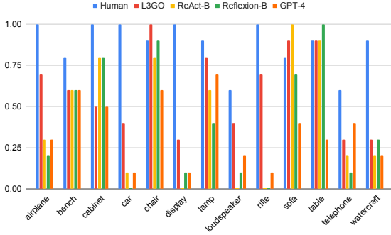
Figure 7: GPT-4V evaluation of L3GO, ReAct-B, Reflexion-B, and GPT-4 on ShapeNet-13. ‘Human’ refers to original ShapeNet meshes that were designed by humans. For complex objects such as airplanes and rifles, L3GO performs better than others.
