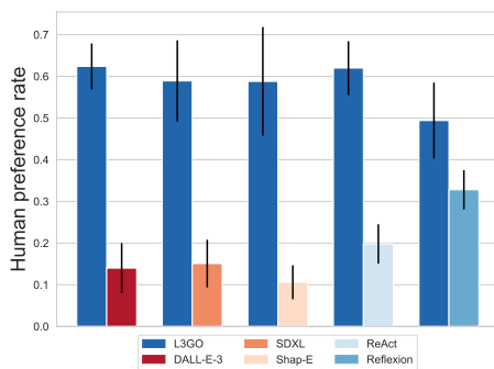
Figure 6: Human preference of L3GO vs. DALL-E-3, SDXL, Shap-E, ReAct-B, and Reflexion-B on UFO.
