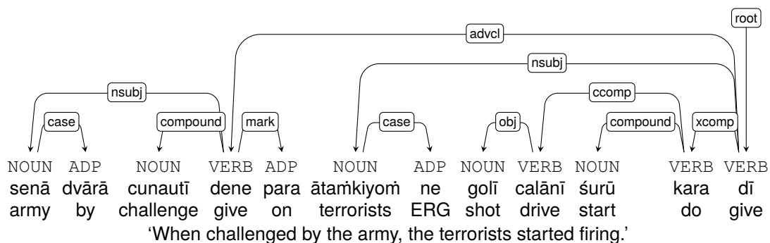
Figure 9: Two verbo-nominal compounds: cunautī denā ‘to challenge’ and śurū karānā ‘to start’. On the other hand, golī calānā ‘to shoot’ is annotated just as a verb-object pair (Hindi HDTB).
