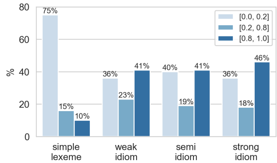
Figure 1: Score distribution
