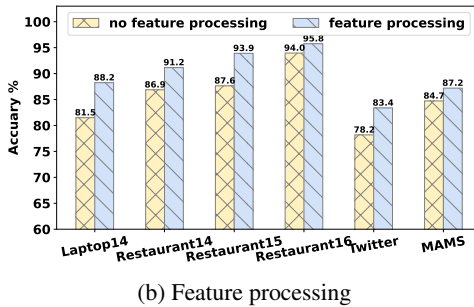
Figure 4: Inference efficiency comparison and the effect of feature processing
