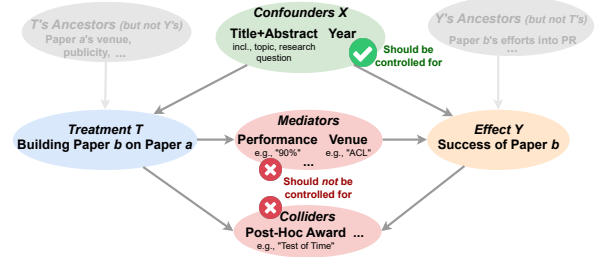
Figure 2: The causal graph of our study.
