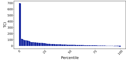
Figure 5: The distribution of TCI values by percentile of 100 random papers, which shows a long tail indicating that high impact is concentrated in a relatively small portion of papers.
