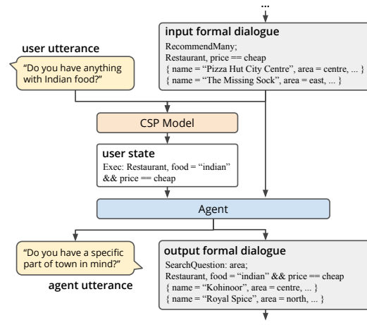
Figure 1: The inference-time flow of a dialogue agent with a contextual semantic parser based on the ThingTalk representation.
