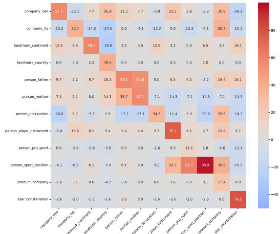
Figure 28: Inter-relation results of the 7B model when considering the neuron type variety as gate_proj .
