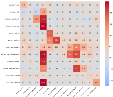
Figure 4: Inter-relation results. Accuracy drops (in %) for the 7B ( left ) and the 13B model ( right ) on \mathcal{P}_{r_i}^{eva} . The number in cell (r_i, r_j) indicates the accuracy drop of relation r_i when deactivating the relation neurons of r_j .
