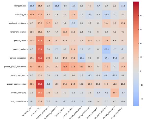
Figure 29: Inter-relation results of the 7B model when considering the neuron type variety as down_proj .
