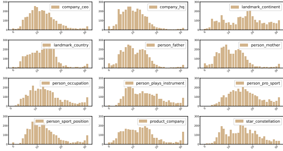
Figure 1: Distribution of RelSpec neurons across layers in the 7B model. Most are located in the middle layers.
