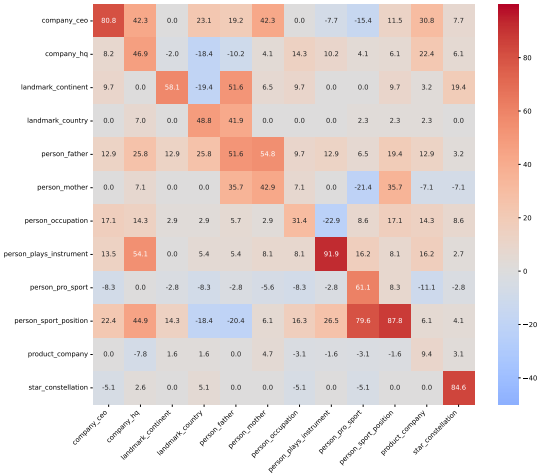
Figure 25: Inter-relation results of the 7B model when considering the neuron type variety as all .
