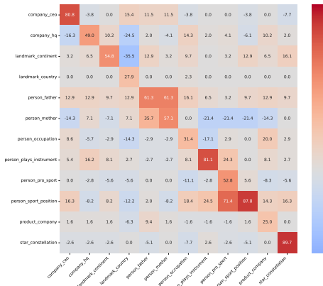
Figure 4: Inter-relation results. Accuracy drops (in %) for the 7B ( left ) and the 13B model ( right ) on \mathcal{P}_{r_i}^{eva} . The number in cell (r_i, r_j) indicates the accuracy drop of relation r_i when deactivating the relation neurons of r_j .
