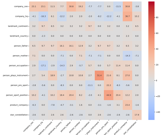
Figure 27: Inter-relation results of the 7B model when considering the neuron type variety as up_proj .
