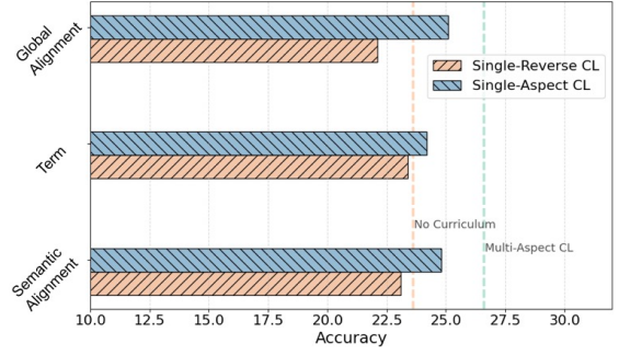
Figure 3: Comparison of Curriculum Learning Strategies.
