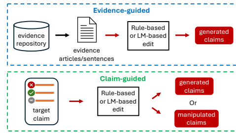
Figure 3: Overview of adversarial claim attacks: evidence-guided and claim-guided.
